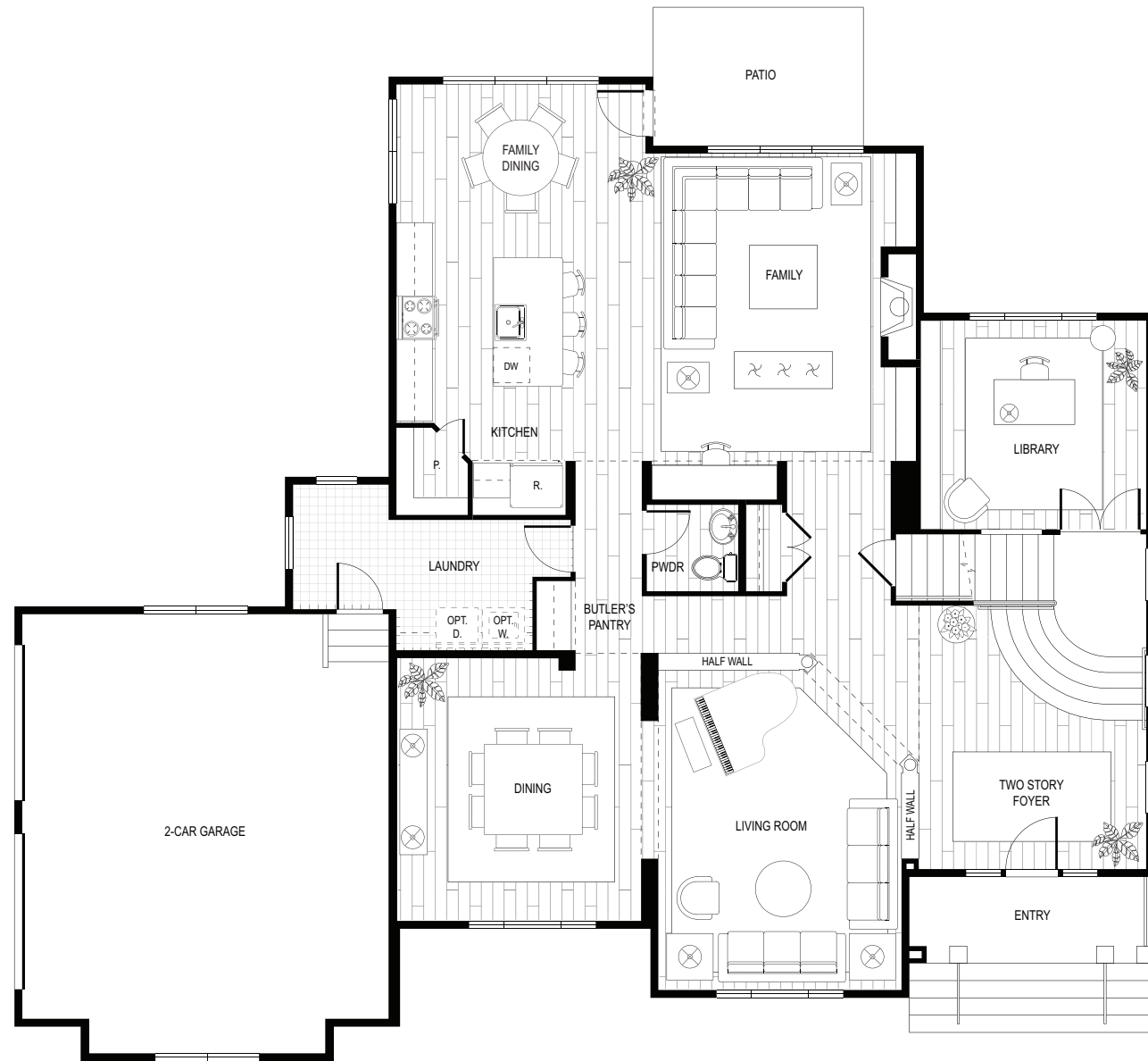
MAIN LEVEL
